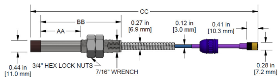
DP100702 Standard Mount
