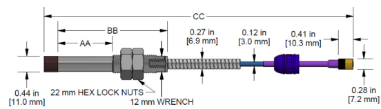
DP100704 Standard Mount
